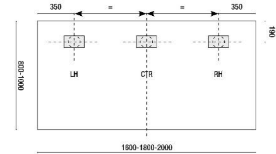
Cable port TYPE "E", "D", "P" and "G"
