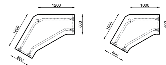
Symmetrical 120° Desk
