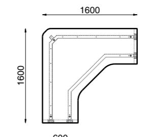
Symmetrical 90° Desk
